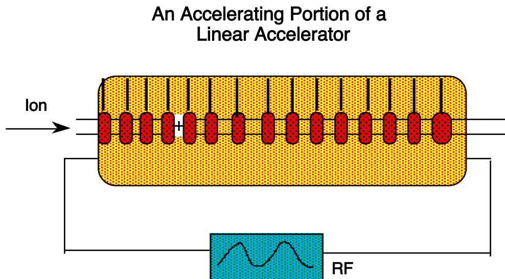
Fig. 11-3. Side view of a linear accelerator. (This figure does not show the increasing spacing between cavities as discussed in the text.)
