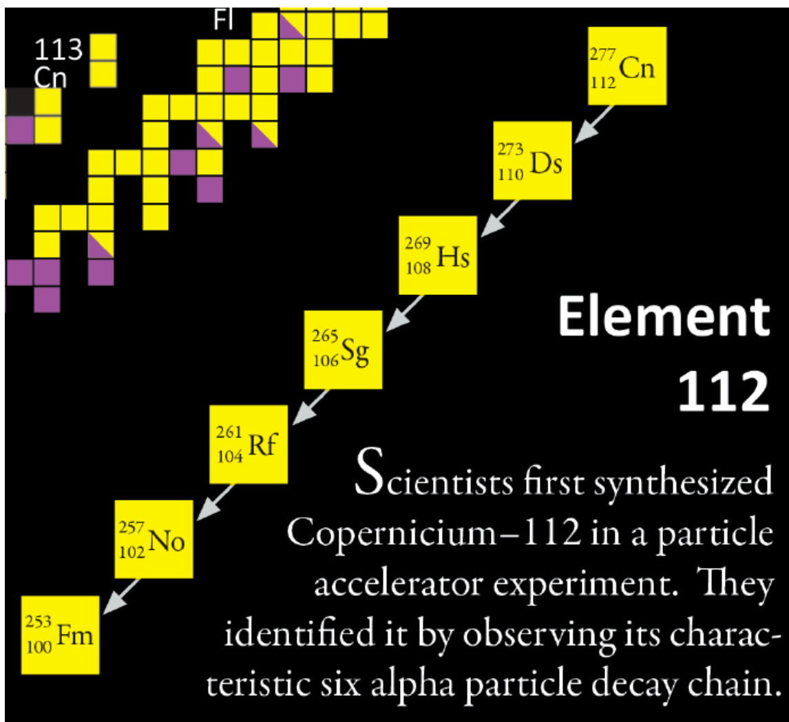
Fig. 8-2. The decay chain for identifying element 112.
